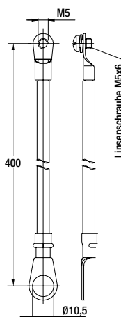
GURO-EC10- R10-400-RM5 (E2)
